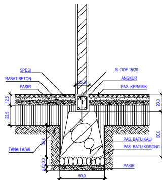
04 DETAIL PONDASI
