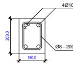
06 DETAIL SLOOF
